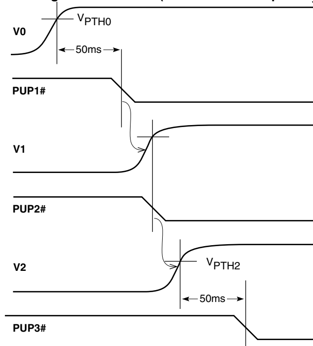
Figure 5. V_x Input and Resulting PUP# Cascade (RESET# set to trip on V_3 Undervoltage)
