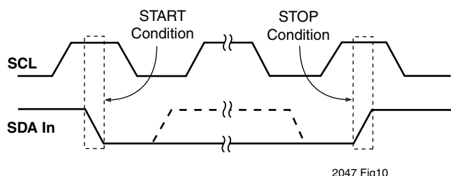
Figure 10. START and STOP Conditions
