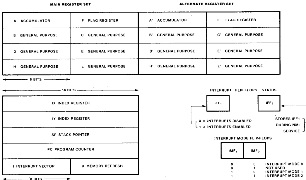
Figure 4. CPU Registers
