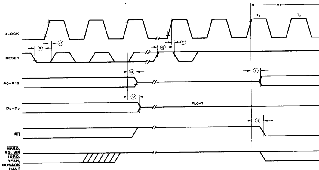
Figure 12. Reset Cycle
