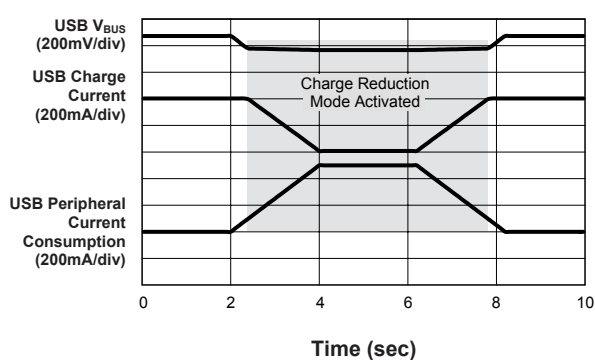
USB Charge Current vs. Time (USBH; USBH = 8.06kΩ)
