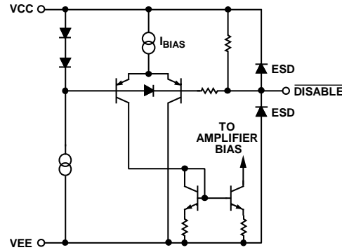
Figure 44. DISABLE Circuit
