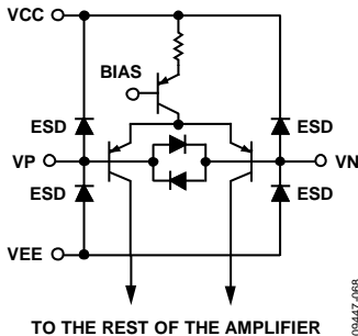
Figure 43. Input Stage and Protection Diodes
