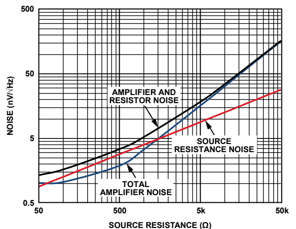
Figure 47. RTI Noise vs. Source Resistance
