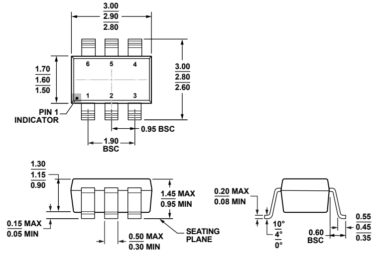
COMPLIANT TO JEDEC STANDARDS MO-178-AB Figure 57. 6-Lead Small Outline Transistor Package [SOT-23] (RJ-6) Dimensions shown in millimeters
