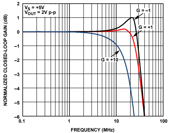
Figure 13. Large Signal Frequency Response vs. Gain
