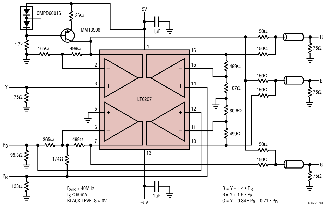
YP B P R to RGB Converter
