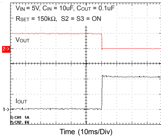
Short Circuit Current Response
