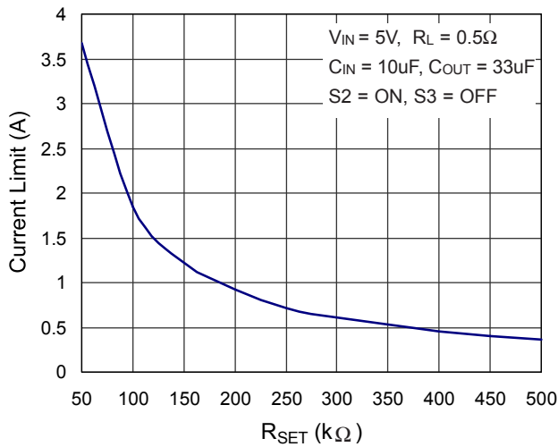
Current Limit vs. R_{SET}
