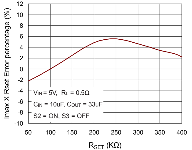
Current Limit Factor vs. R_{SET}
