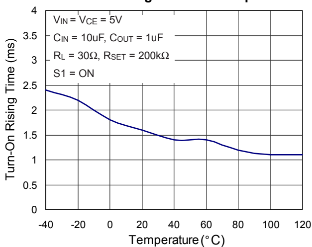
① Turn-On Rising Time vs. Temperature
