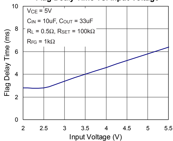
④ Flag Dealy Time vs. Input Voltage
