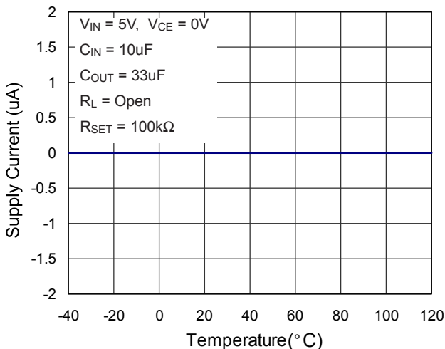
② Off-State Supply Current vs. Temperature
