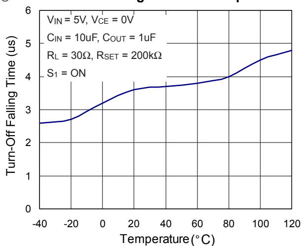
① Turn-Off Falling Time vs. Temperature
