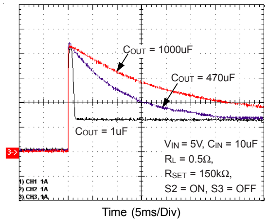
Inrush Current Response
