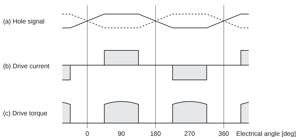
Fig. 5. Operating Waveforms of a DDC System Single-phase Full Wave Drive Type Driver
