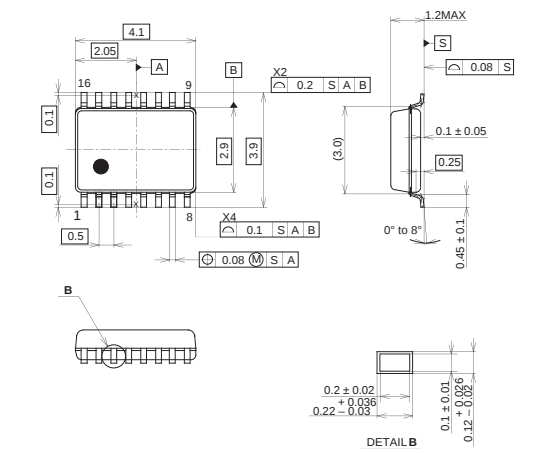
16PIN TSSOP(PLASTIC)
