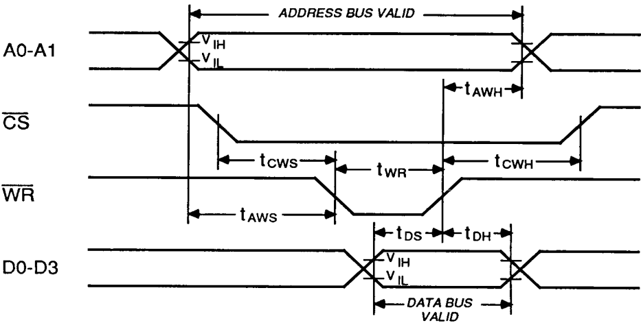
TIMING MEASUREMENT REFERENCE LEVEL IS (VIH + VIL)/2 UNLESS OTHERWISE INDICATED
