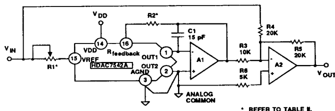
FIGURE 6 BIPOLAR OPERATION
