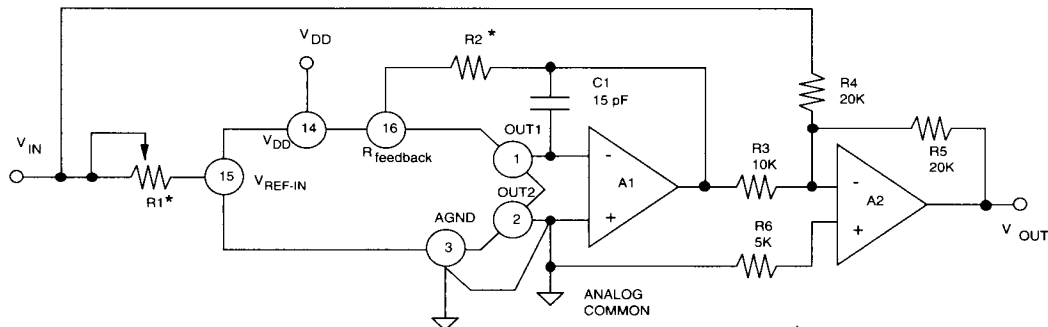
Figure 7 - Bipolar Operation
