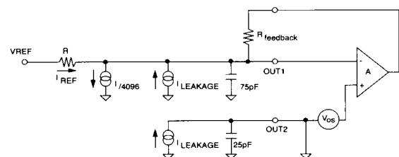
Figure 4 - HDAC7542A DAC Equivalent Circuit All Digital Inputs High
