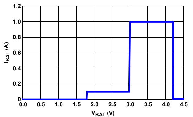
FIGURE 25. BATTERY CURRENT vs BATTERY VOLTAGE (CC MODE)
