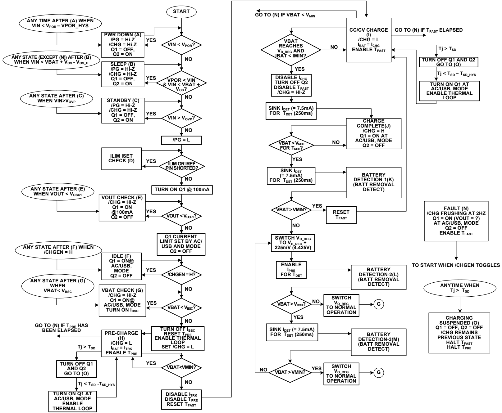
FIGURE 31. STATE DIAGRAM
