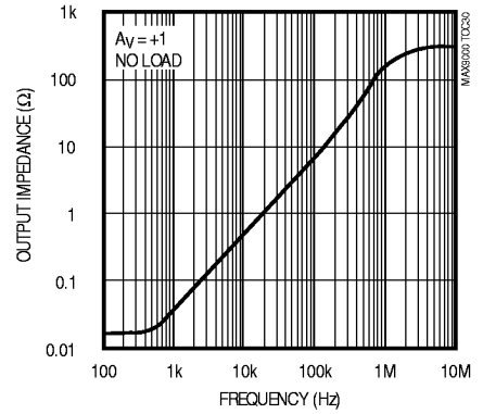
MAX9000/MAX9001/MAX9002 OP-AMP OUTPUT IMPEDANCE vs. FREQUENCY
