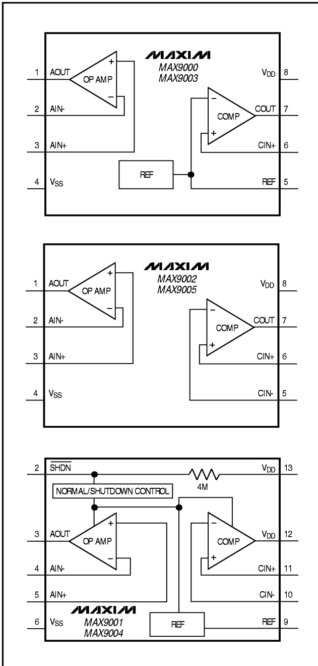
Figure 1. MAX9000–MAX90005 Functional Diagrams
