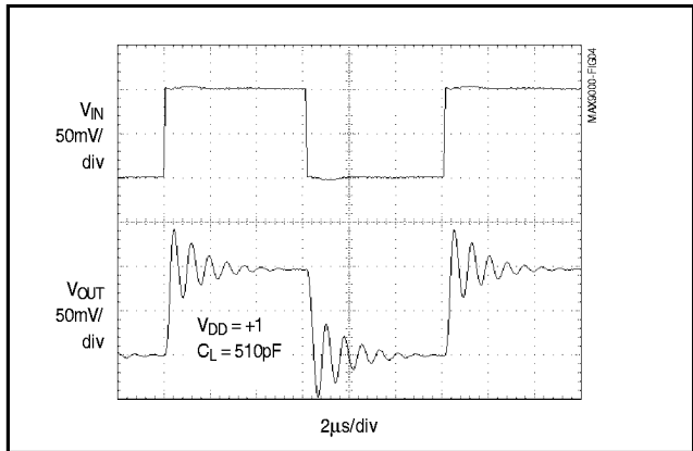
Figure 4. MAX9000/MAX9001/MAX9002 Op-Amp Small-Signal Transient Response with Capacitive Load ( C_L = 510\text{pF} ) and No Isolation Resistor
