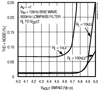
MAX9003/MAX9004/MAX9005 OP-AMP TOTAL HARMONIC DISTORTION PLUS NOISE vs. V_{AOUT}
