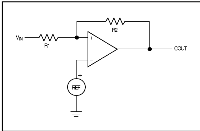
Figure 6. External Hysteresis
