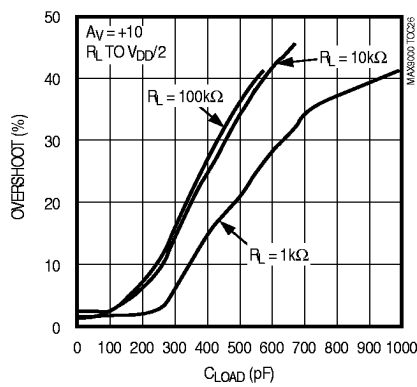
MAX9003/MAX9004/MAX9005 OP-AMP PERCENT OVERSHOOT vs. LOAD CAPACITANCE
