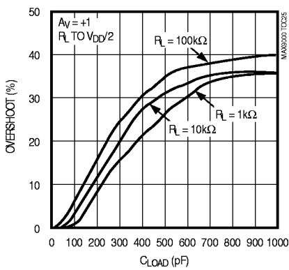
MAX9000/MAX9001/MAX9002 OP-AMP PERCENT OVERSHOOT vs. LOAD CAPACITANCE
