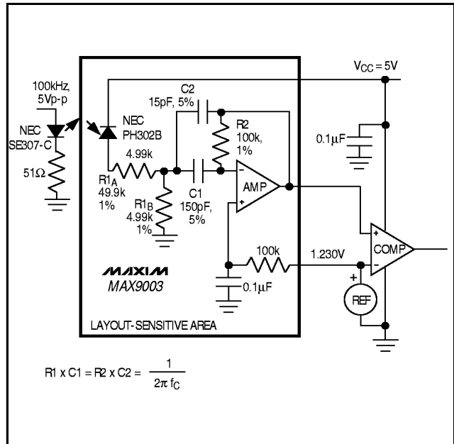
Figure 9. Infrared Receiver Application
