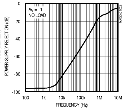
MAX9003/MAX9004/MAX9005 OP-AMP POWER-SUPPLY REJECTION vs. FREQUENCY
