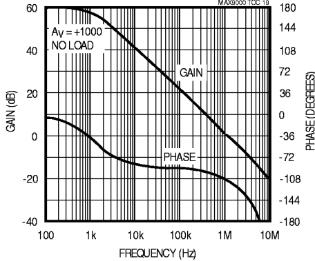
MAX9003/MAX9004/MAX9005 OP-AMP GAIN AND PHASE vs. FREQUENCY (NO LOAD)
