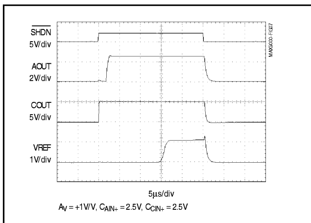
Figure 7. Enable/Disable Response of Op Amp, Comparator, and Reference to \overline{SHDN}
