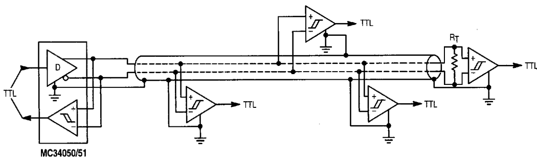
Figure 17. EIA-423 Application
