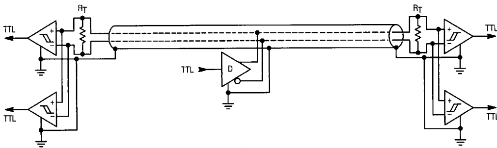
Figure 17. EIA-423 Application
