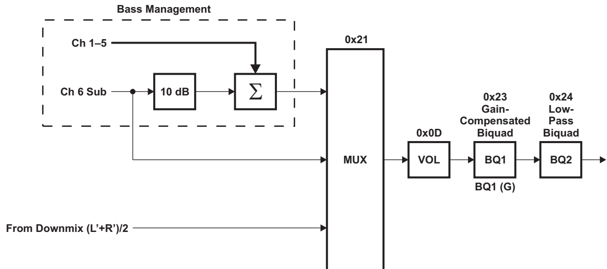
Figure 3. Channel-6 Processing Block Diagram
