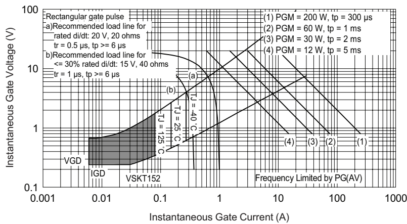
Fig. 12 - Gate Characteristics
