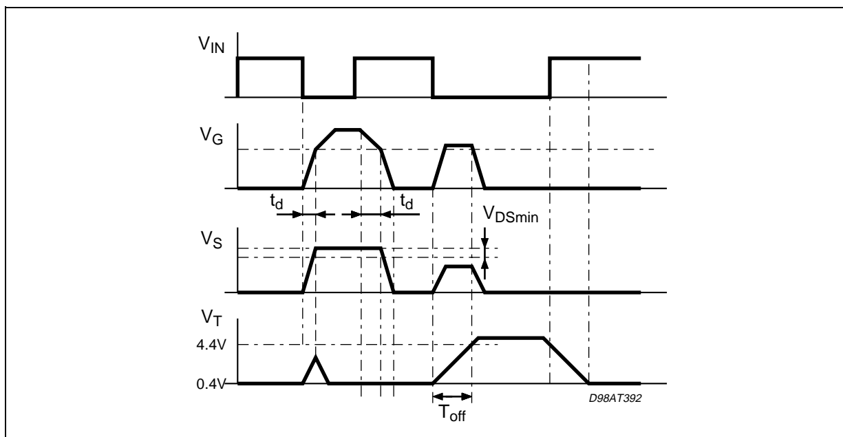
Figure 1. Timing Characteristic.
