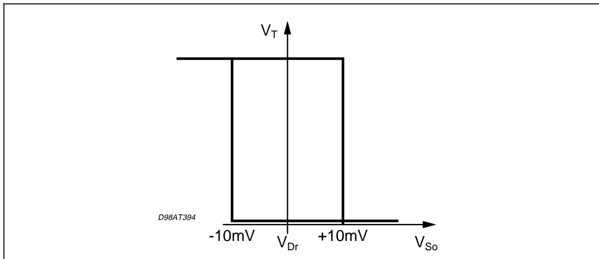
Figure 3. Comparator hysteresis
