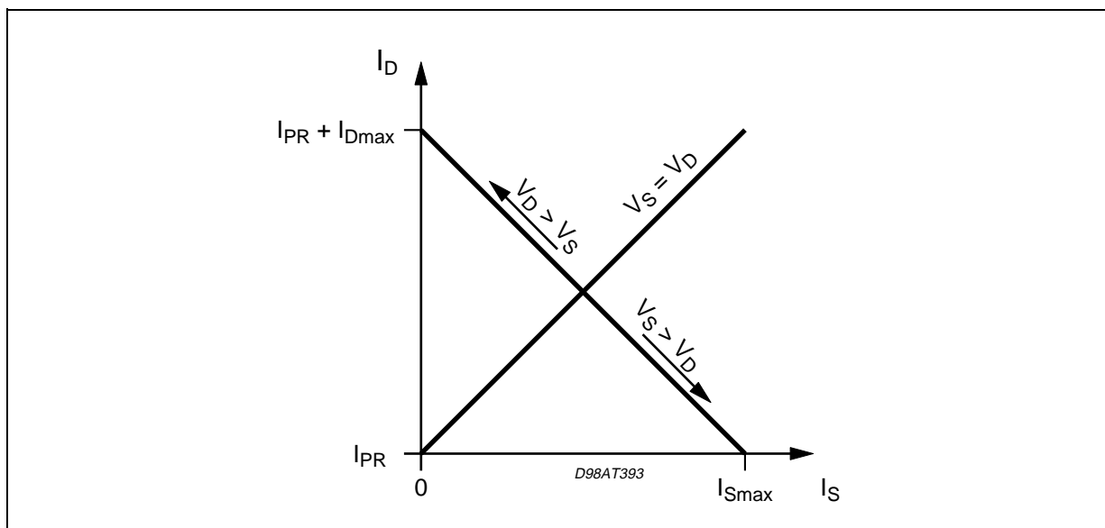
Figure 2. Drain, source input current.
