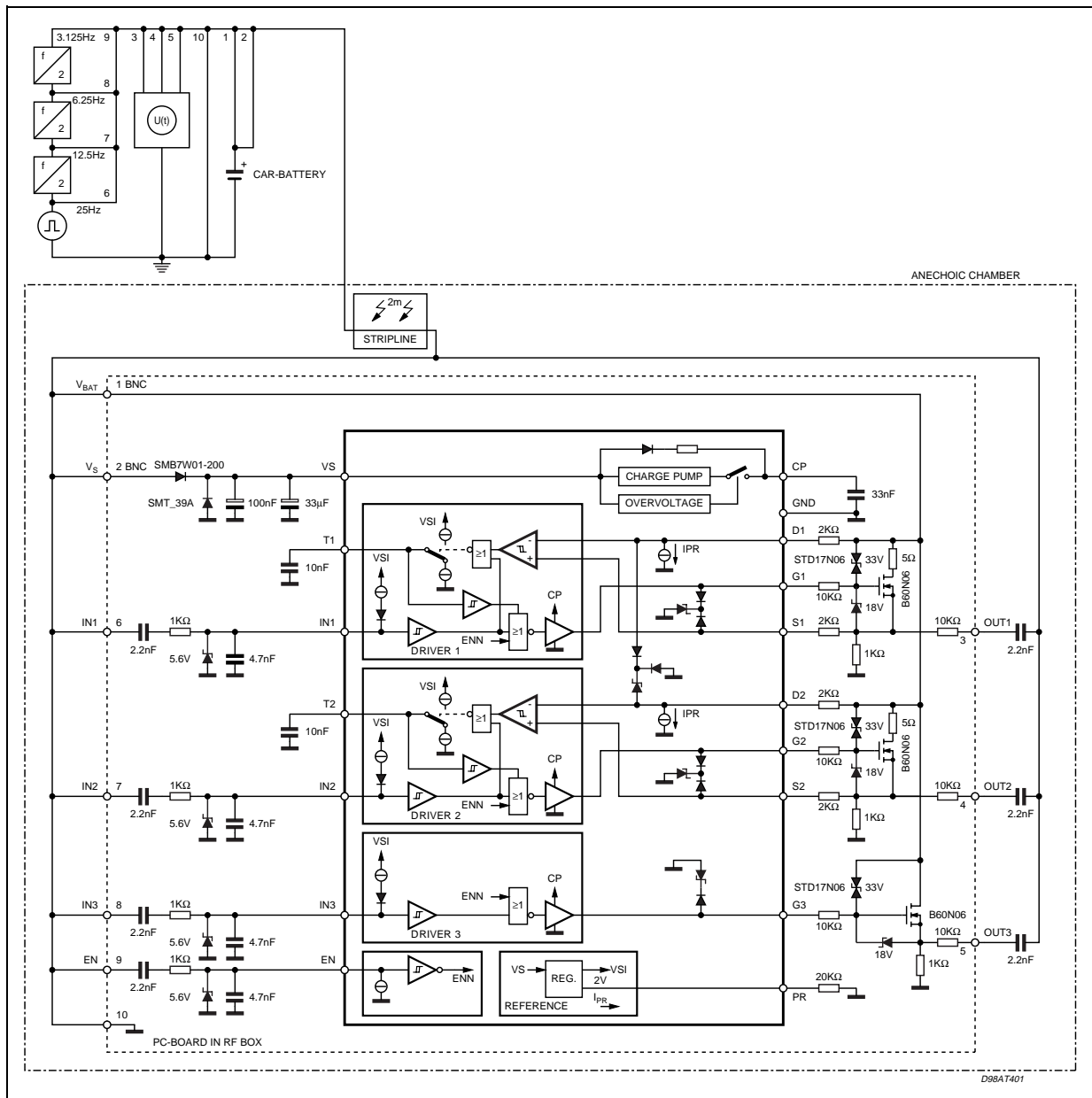
Figure 10. Measured Circuit
