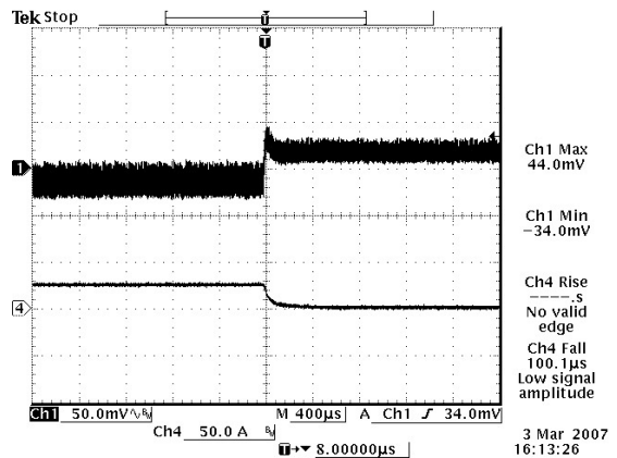
Vout=1.2 V 50%-0% Load Transient
