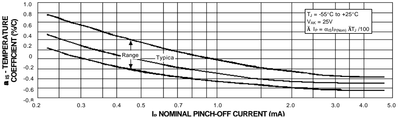
Temperature Coefficient
