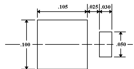
Mounting Pad Dimensions in Inches
