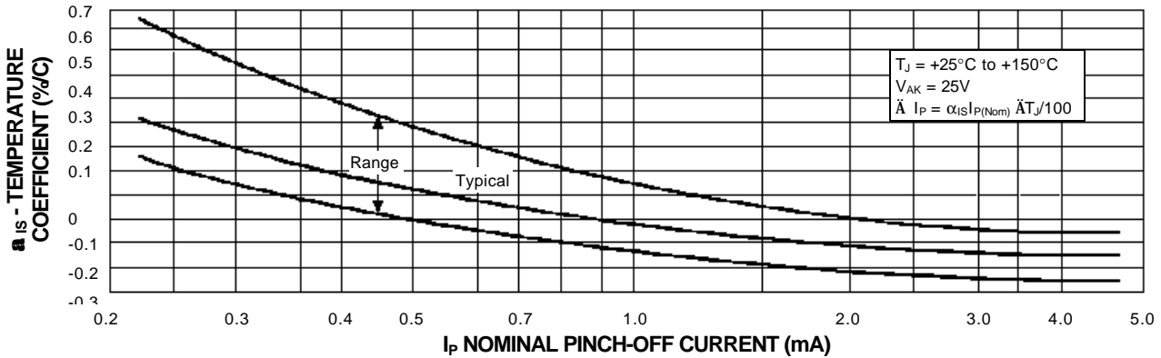
Temperature Coefficient
