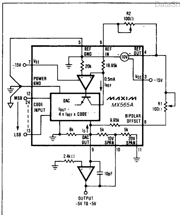
Figure 4(b). MX565A ±5V Bipolar Voltage Output
