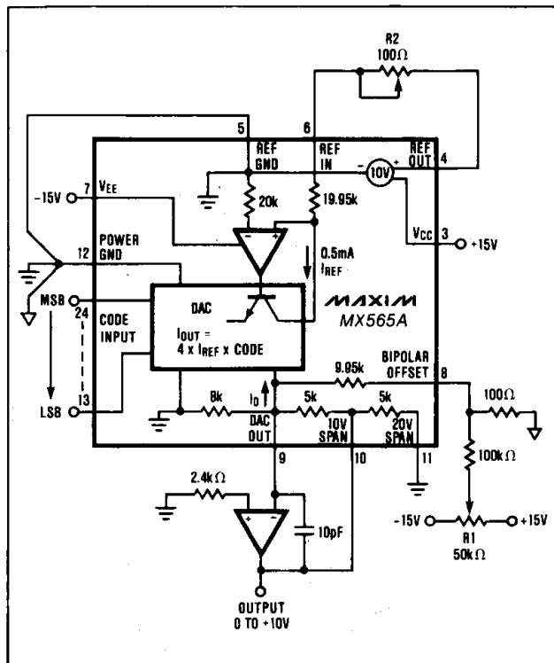
Figure 4(a). MX565A 0 to +10V Unipolar Voltage Output
