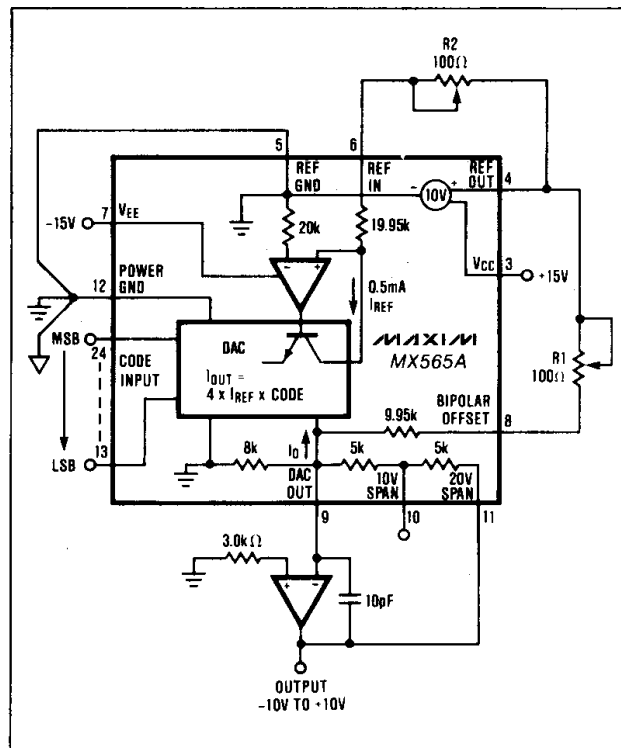
Figure 4(c). MX565A ±10V Bipolar Voltage Output
