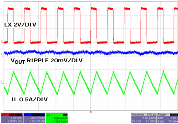
www.DataSheet4U.com FIGURE 17. STEADY STATE OPERATION AT NO LOAD (PWM)
