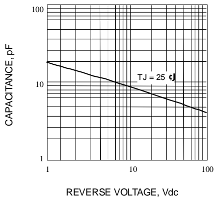
Fig. 4-TYPICAL JUNCTION CAPACITANCE
