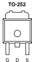
Top View Order Number: SUD50N02-12P
