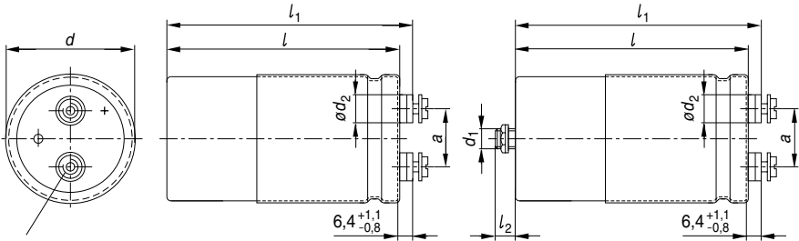
Type B43750 Ring clip/clamp mounting
