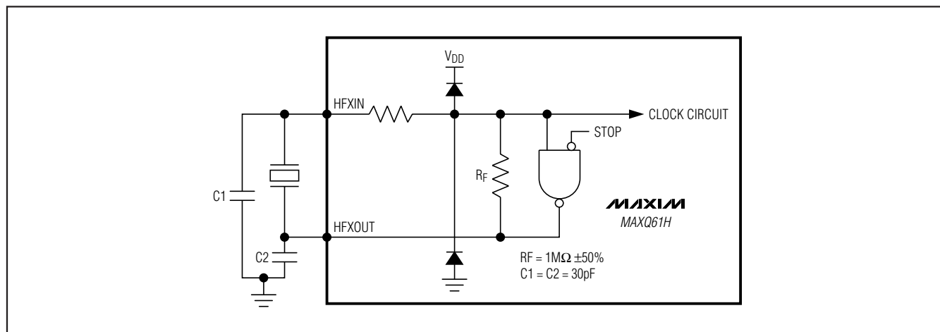
Figure 7. On-Chip Oscillator
