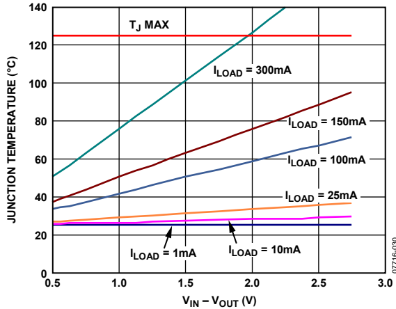
Figure 35. 0 mm 2 of PCB Copper, T_A = 25^\circ\text{C}
