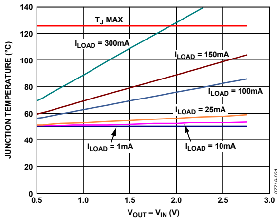
Figure 36. 500 mm 2 of PCB Copper, T_A = 50^\circ\text{C}
