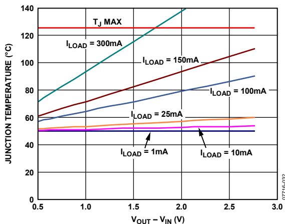
Figure 37. 100 mm 2 of PCB Copper, T_A = 50^\circ\text{C}
