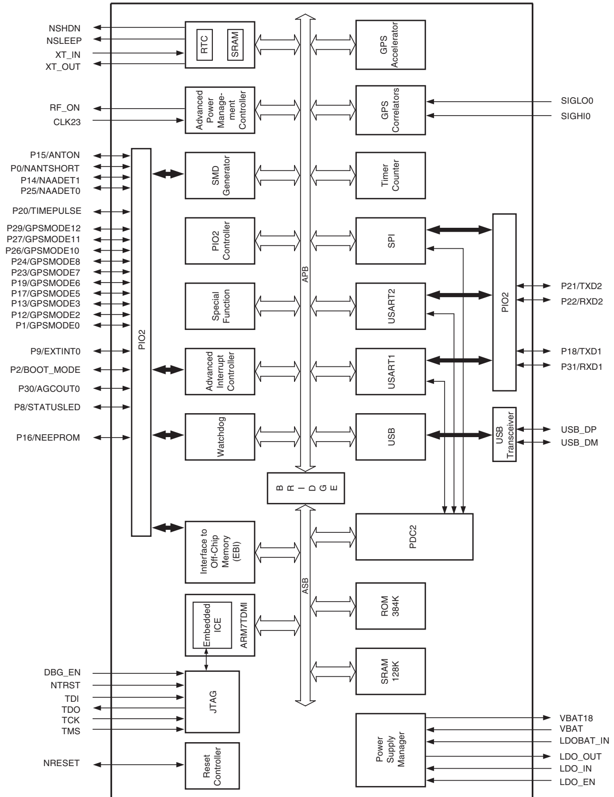
Figure 1-1. ATR0622 Block Diagram
