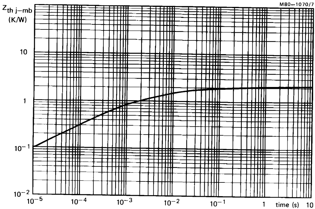
Fig.11 Transient thermal impedance.
