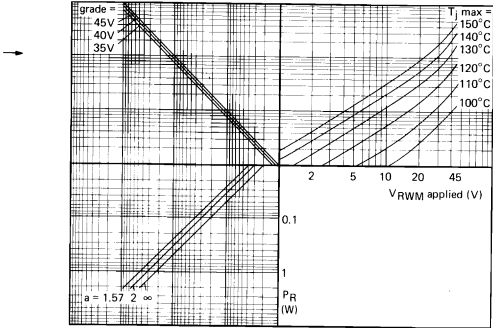
Fig.5 NOMOGRAM: for calculation of P_R (reverse leakage power dissipation) for a given T_j \text{ max.} , V_{RWM} applied, voltage grade and form factor.
