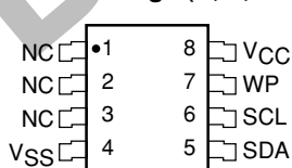
MSOP Package (R, Z, GZ)
