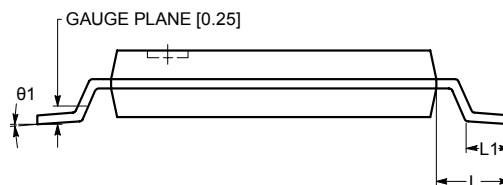
END VIEW
