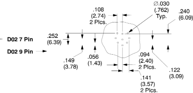
PC Board Layout for D02EEB906FD21TABH
