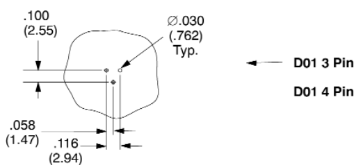
PC Board Layout for D01EEB306FD21TABH
