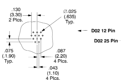
PC Board Layout for D02EEB125FD21TABH
