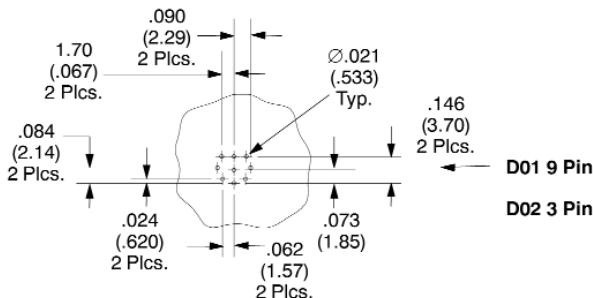
PC Board Layout for D01EEB904FD21UTABH
