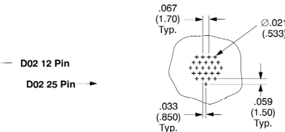
PC Board Layout for D02EEB2504FD21UTABH
