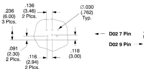
PC Board Layout for D02EEB706FD21TABH
