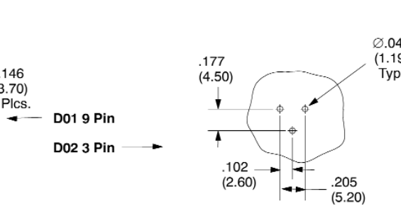
PC Board Layout for D02EEB315FD21TABH
