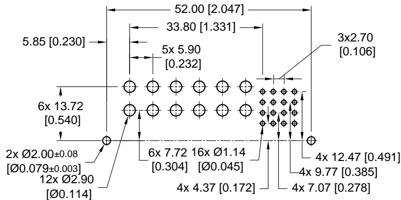
CONTACT HOLES PATTERN
