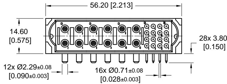
CONTACT HOLES PATTERN
