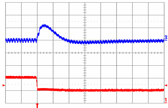
Fig. 1.8V.8: Output voltage response (YNL12S10018) to negative load current step change from 10 A to 5 A with slew rate of -5 A/ \mu\text{s} at V_{in} = 12\text{ V} . Top trace: output voltage (100 mV/div.); Bottom trace: load current (5 A/div.). C_o = 100\text{ }\mu\text{F} ceramic. Time scale: 20 \mu\text{s} /div.
