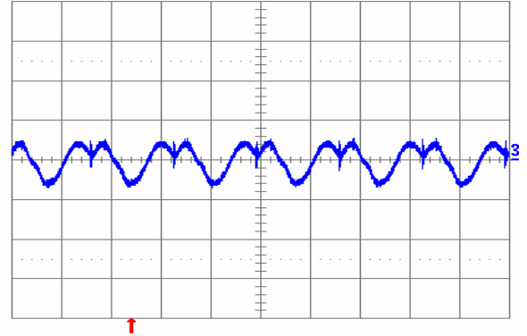
Fig. 1.8V.6: Output voltage ripple (20 mV/div.) at full rated load current into a resistive load with external capacitance 100 \mu\text{F} ceramic + 1 \mu\text{F} ceramic and V_{in} = 12\text{ V} (YNL12S10018). Time scale: 2 \mu\text{s} /div.
