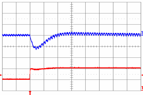
Fig. 1.8V.7: Output voltage response (YNL12S10018) to positive load current step change from 5 A to 10 A with slew rate of 5 A/ \mu\text{s} at V_{in} = 12\text{ V} . Top trace: output voltage (100 mV/div.); Bottom trace: load current (5 A/div.). C_o = 100\text{ }\mu\text{F} ceramic. Time scale: 20 \mu\text{s} /div.
