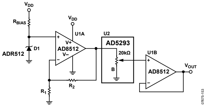
Figure 51. High Voltage DAC
