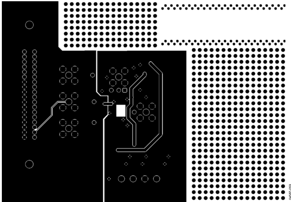
Figure 67. Solder-Side Artwork
