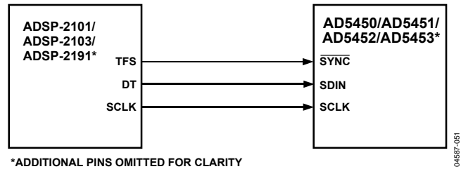
Figure 57. ADSP-2101/ADSP-2103/ADSP-2191 SPORT-to-AD5450/AD5451/AD5452/AD5453 Interface
