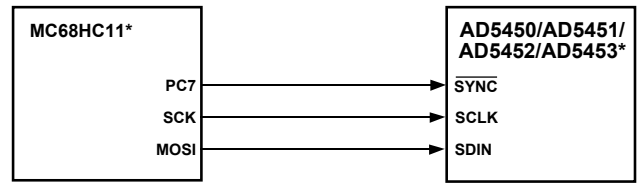
Figure 61. MC68HC11-to-AD5450/AD5451/AD5452/AD5453 Interface
