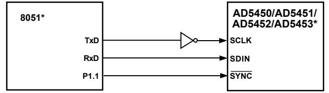
Figure 60. 80C51/80L51-to-AD5450/AD5451/AD5452/AD5453 Interface
