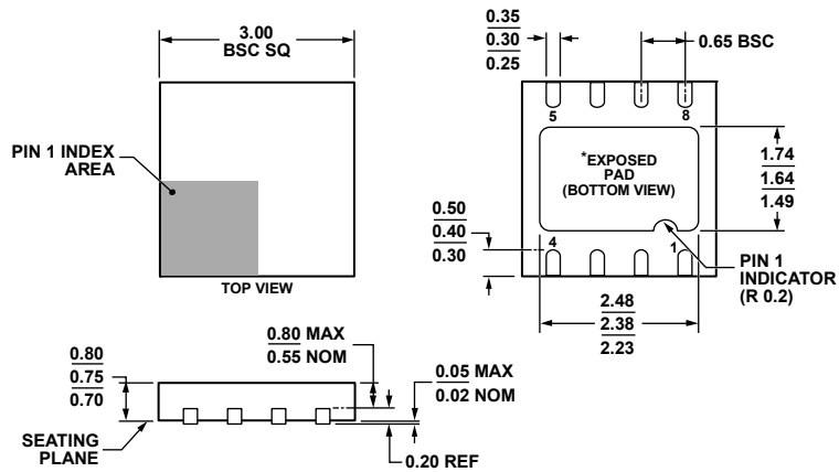
Figure 70. 8-Lead Lead Frame Chip Scale Package [LFCSP_WD] 3 mm x 3 mm Body, Very Very Thin, Dual Lead (CP-8-3)
