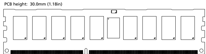
Figure 1: 240-Pin RDIMM (MO-269 R/C C)
