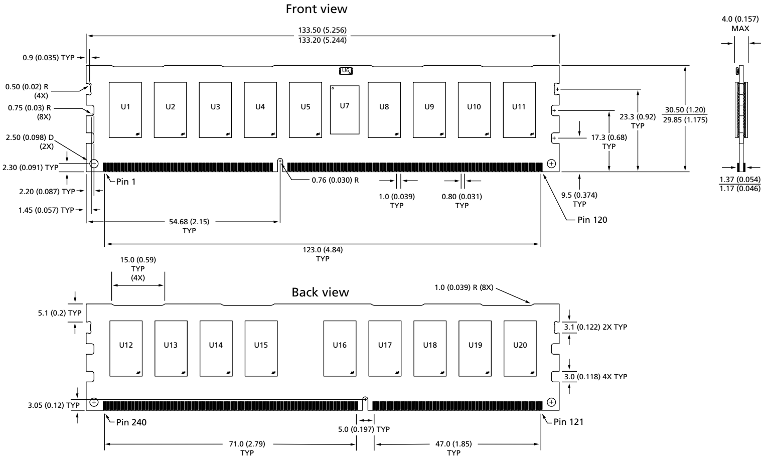
Figure 5: 240-Pin DDR3 RDIMM
