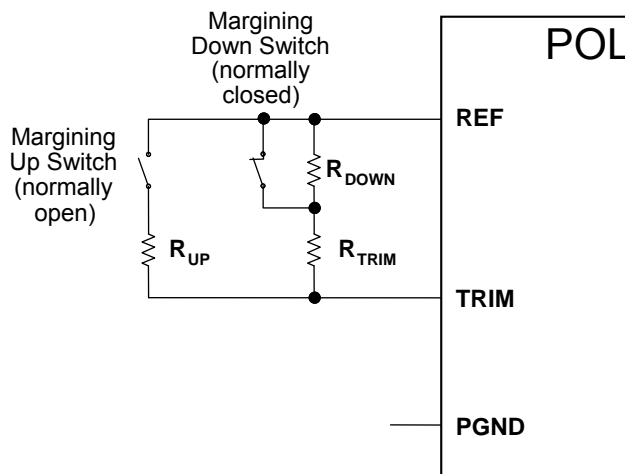
Figure 19. Margining Configuration
