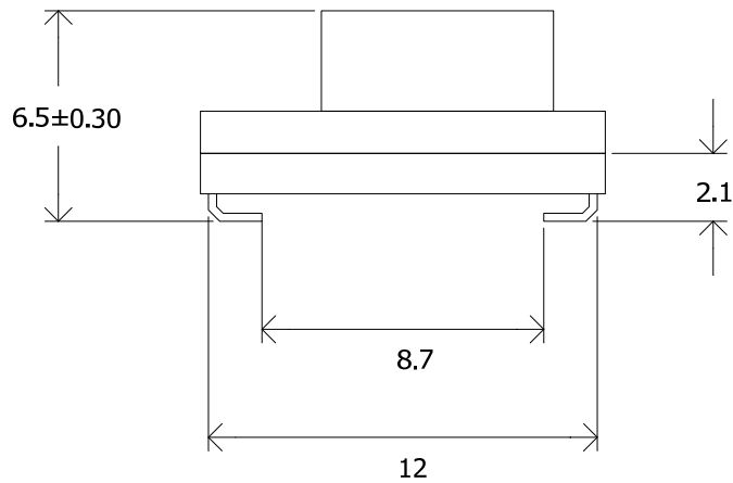
Figure 22. Side View
