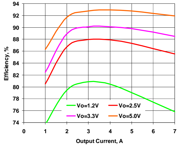
Figure 4. Efficiency vs. Load. Vin=9.6V
