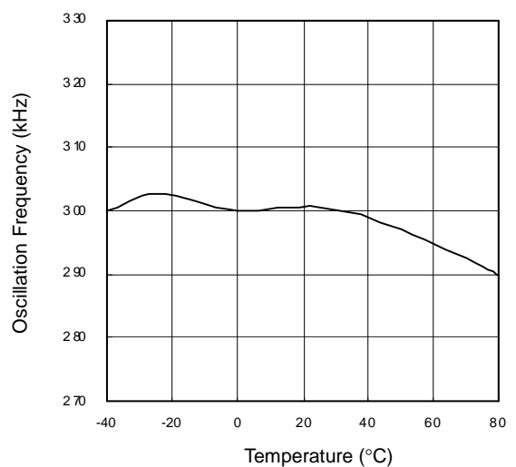
Oscillation Frequency vs. Temperature
