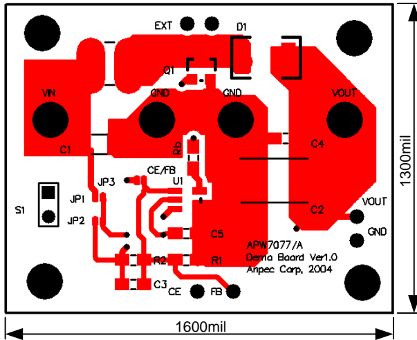
Top Layout
