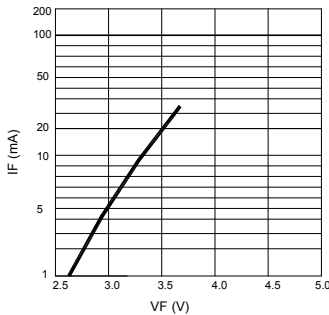
Fig.1 IF-VF Characteristics
