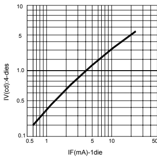
Fig.3 IV-IF Characteristics
