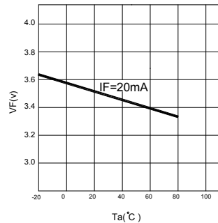
Fig.2 VF-Ta Characteristics
