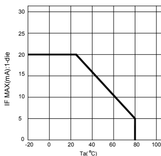
Fig.5 Max-Ta Characteristics
