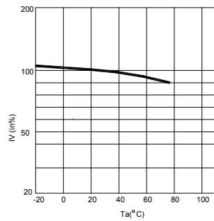
Fig.4 IV-Ta Characteristics
