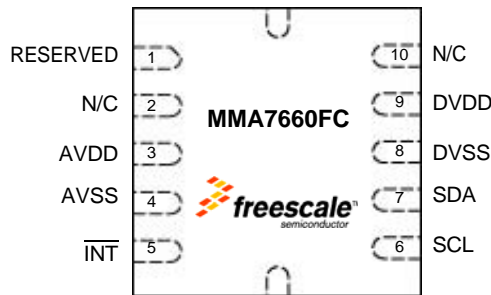
Figure 1. Pin Connections
