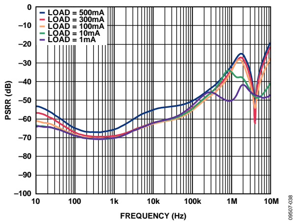
Figure 43. Power Supply Rejection Ratio vs. Frequency, V_{OUT} = 5 V , V_{IN} = 6 V Adjustable With Noise Reduction Circuit
