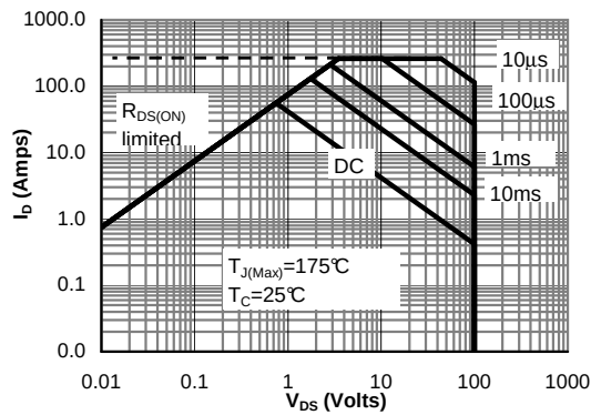
Figure 9: Maximum Forward Biased Safe Operating Area for AOTF2918L (Note F)
