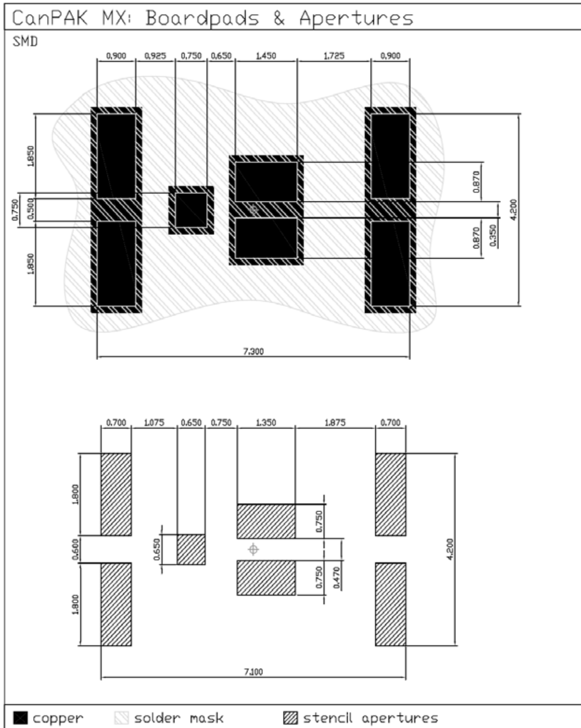
Figure 3 Outlines MG-WDSO-2, dimensions in mm/inches
