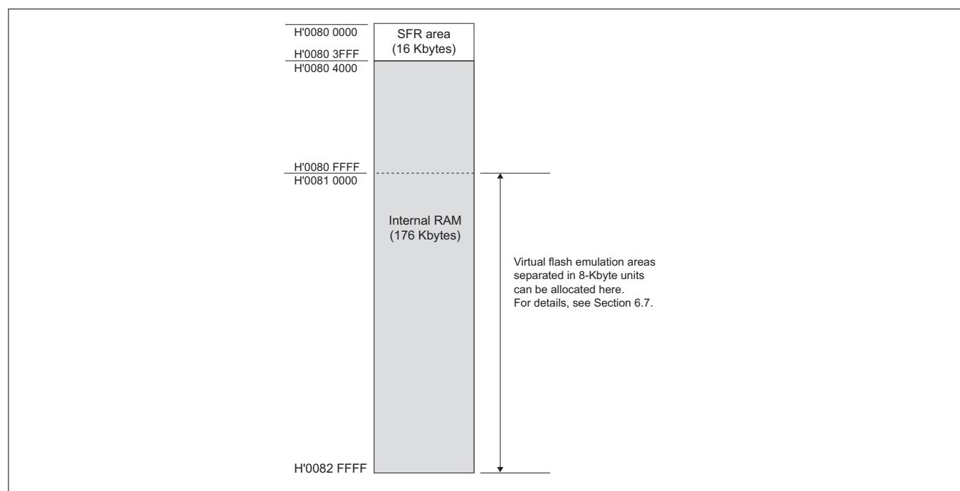
Figure 3.4.1 Internal RAM and SFR (Special Function Register) Areas of the M32192F8
