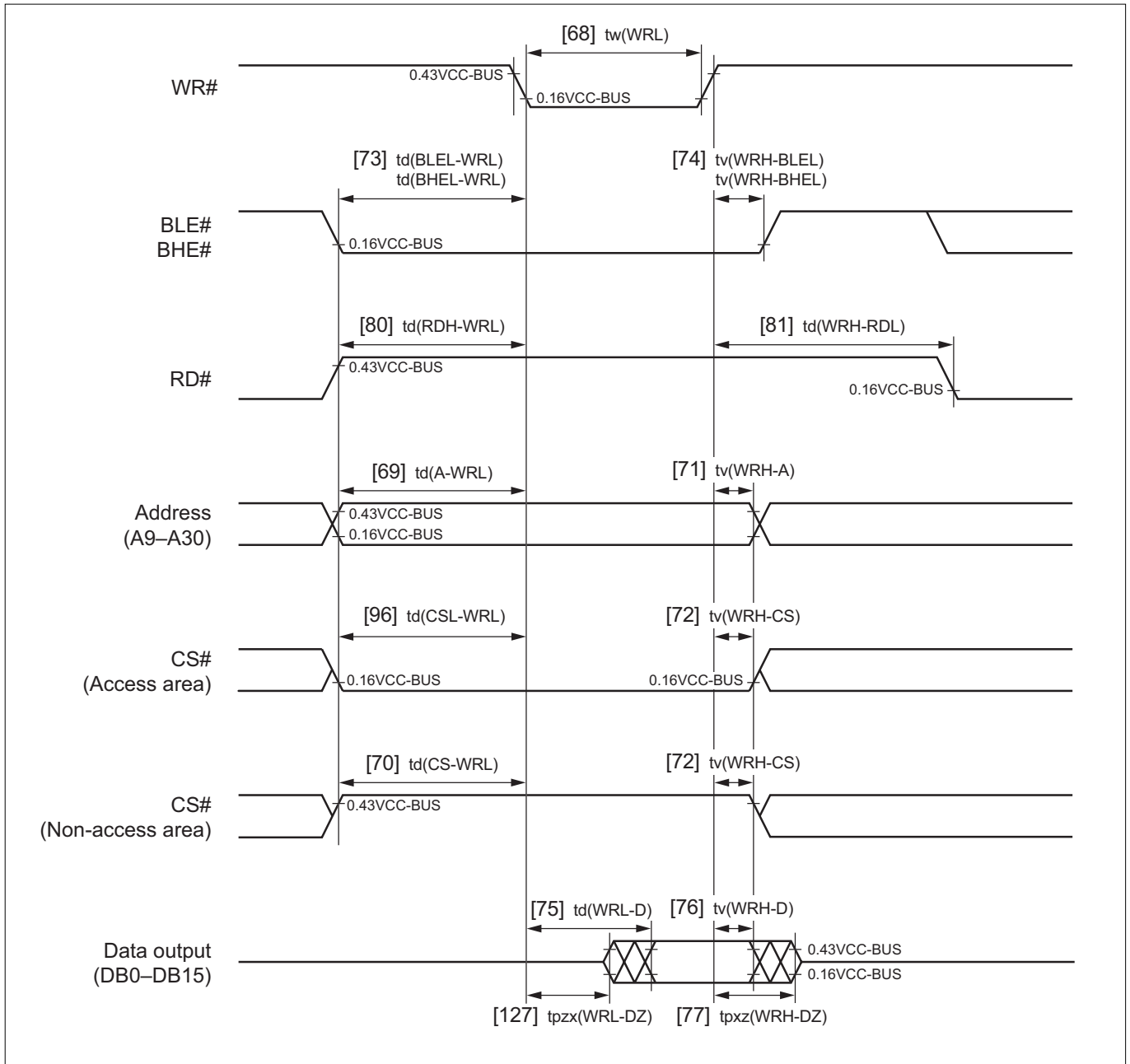
Figure 23.9.15 Write Timing (Byte Enable Mode)
