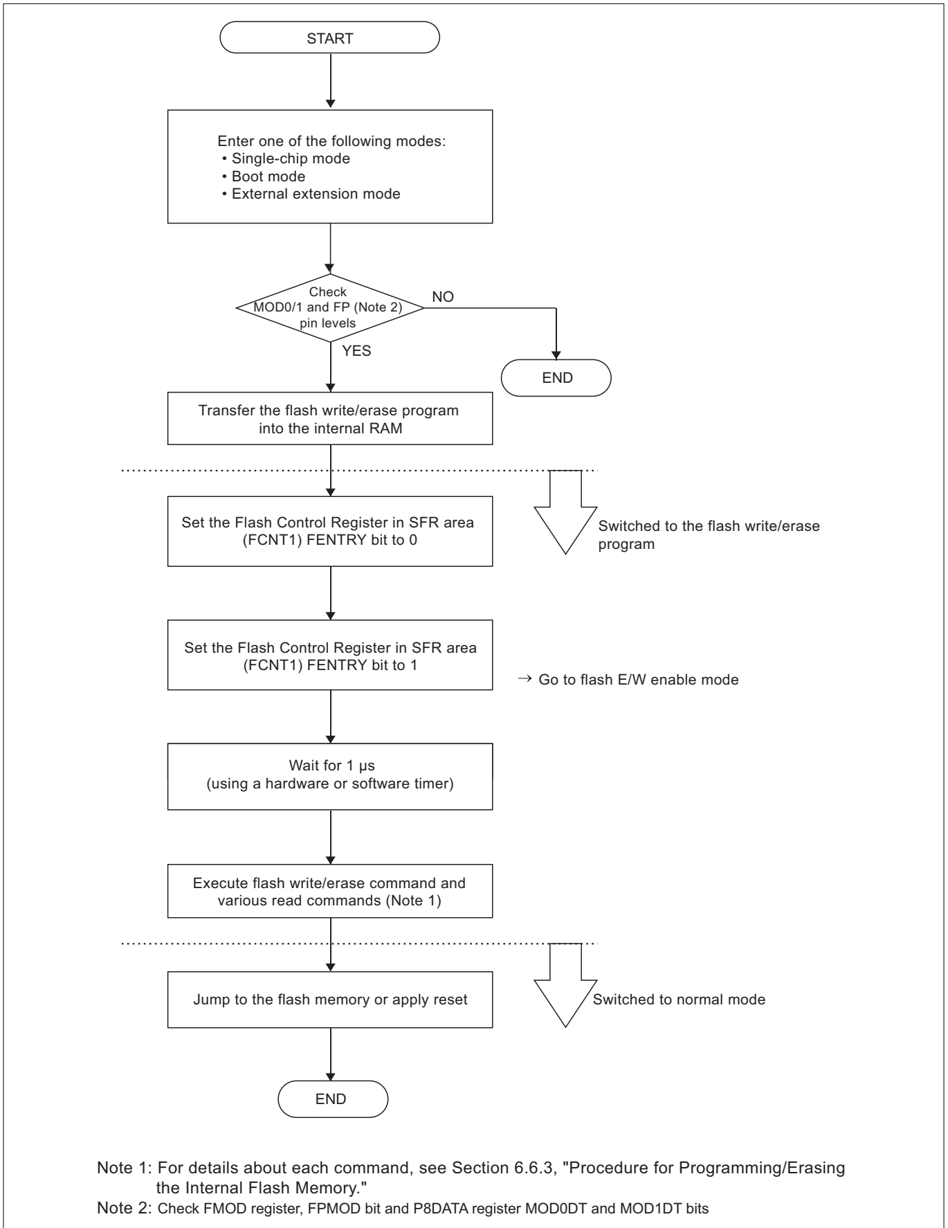
Figure 6.6.6 Procedure for Entering Flash E/W Enable Mode
