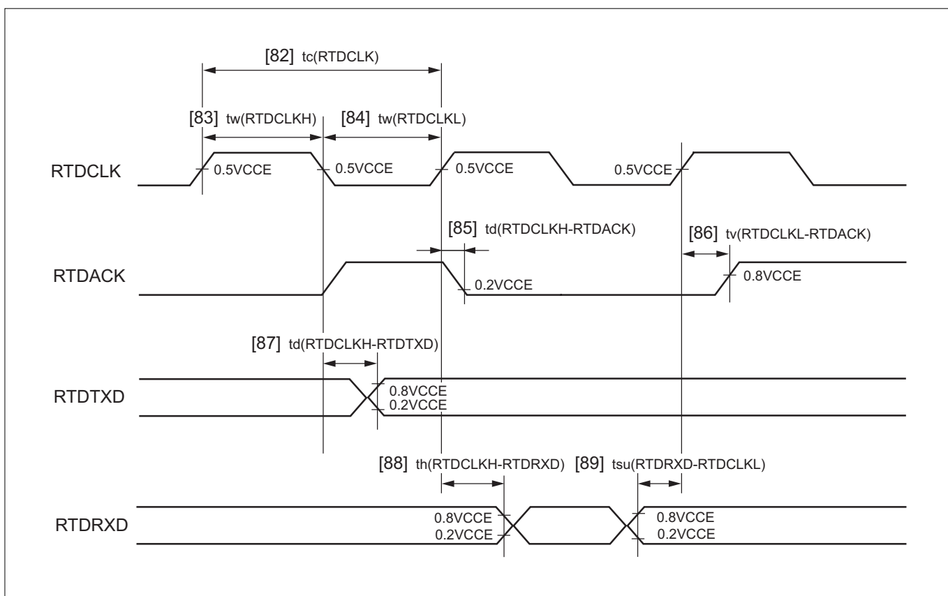
Figure 23.9.18 RTD Timing
