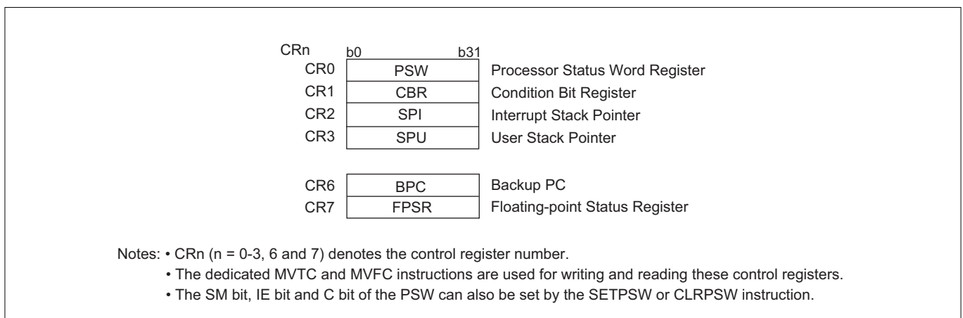
Figure 2.3.1 Control Registers
