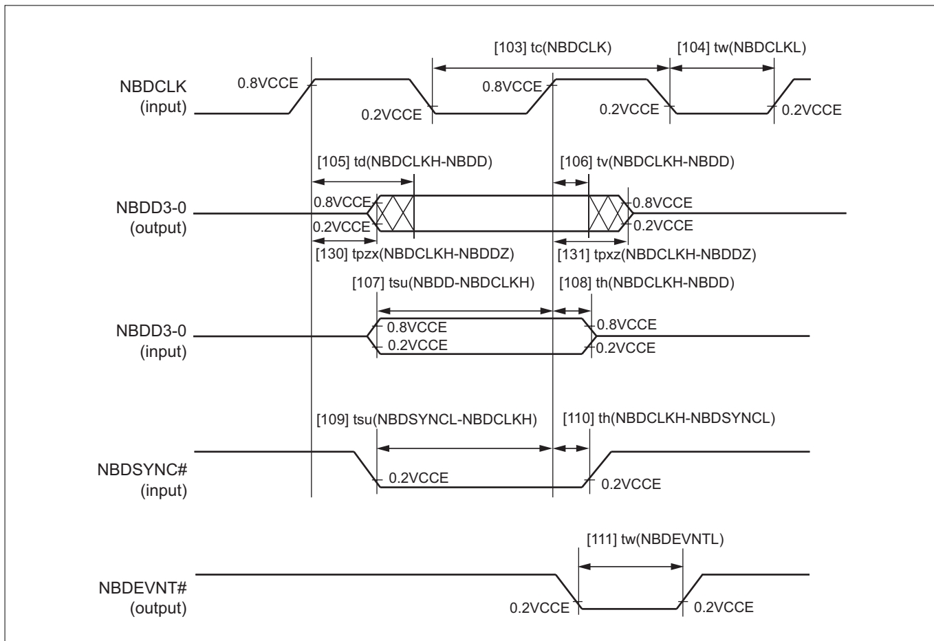
Figure 23.10.19 NBD Timing
