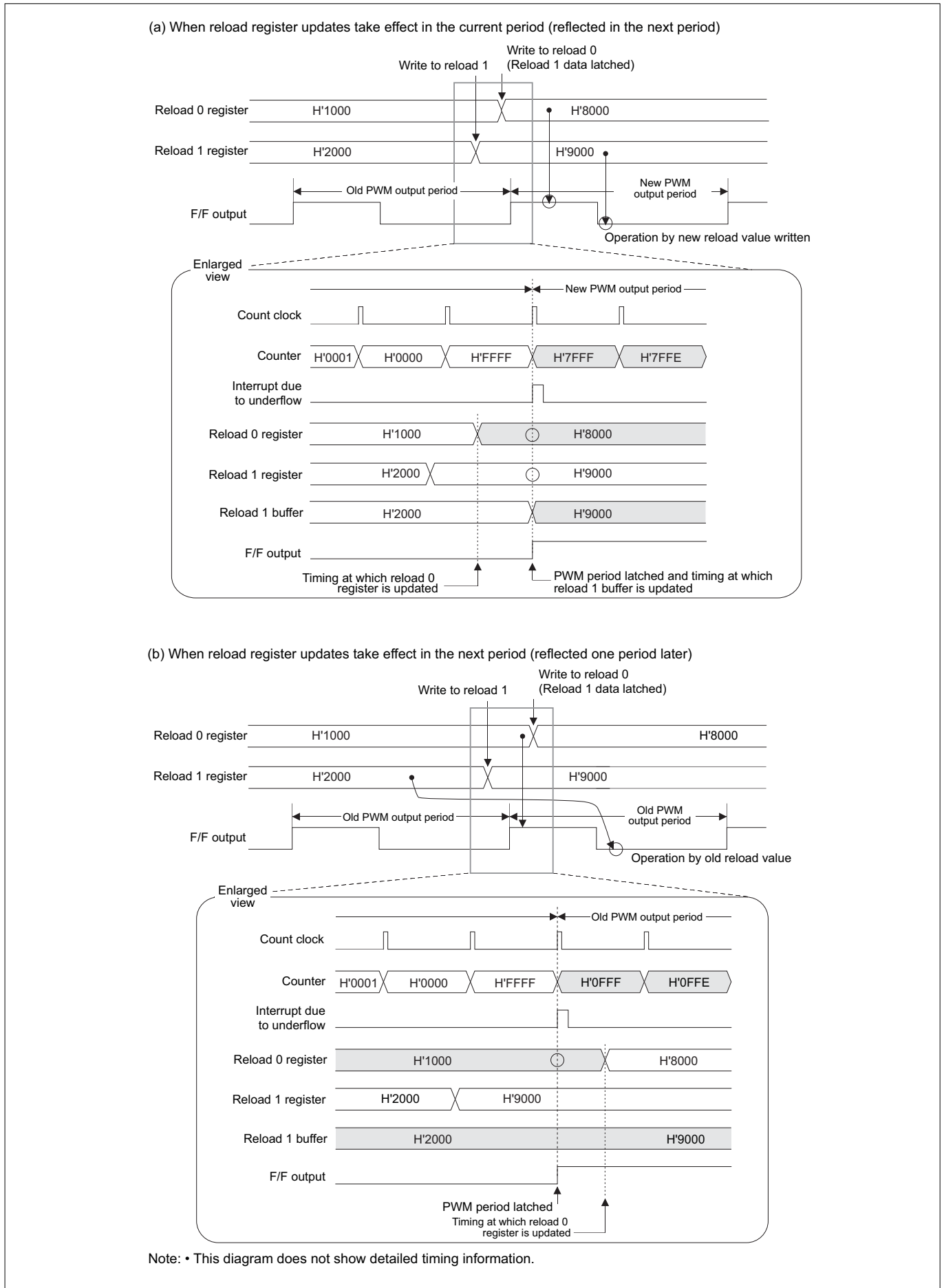
Appendix Figure 4.9.4 Reload 0 and Reload 1 Register Updates in PWM Output Mode
