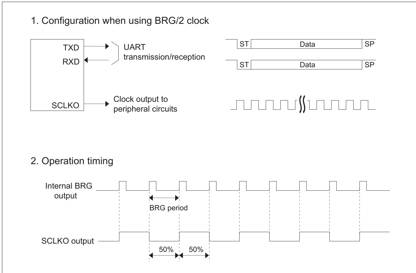
Figure 12.8.1 Example of Fixed Period Clock Output
