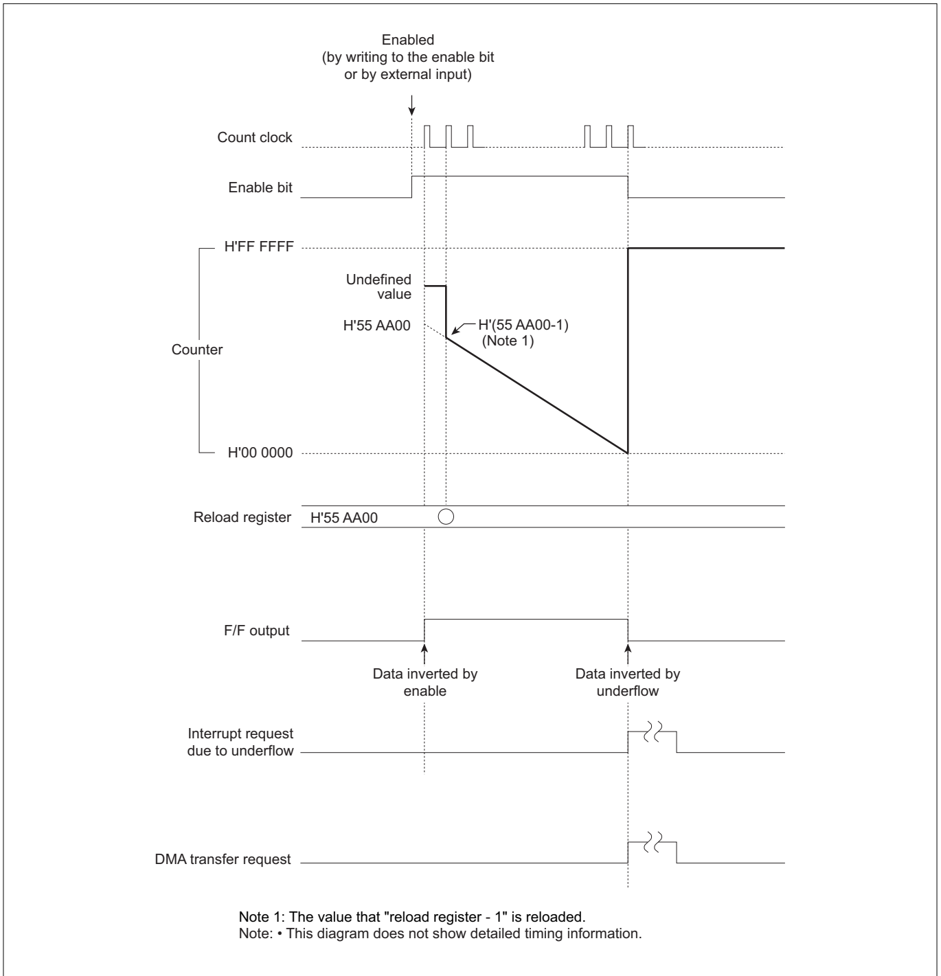
Figure 10.8.14 Typical Operation in TOU Single-shot Output Mode (without Correction Function)
