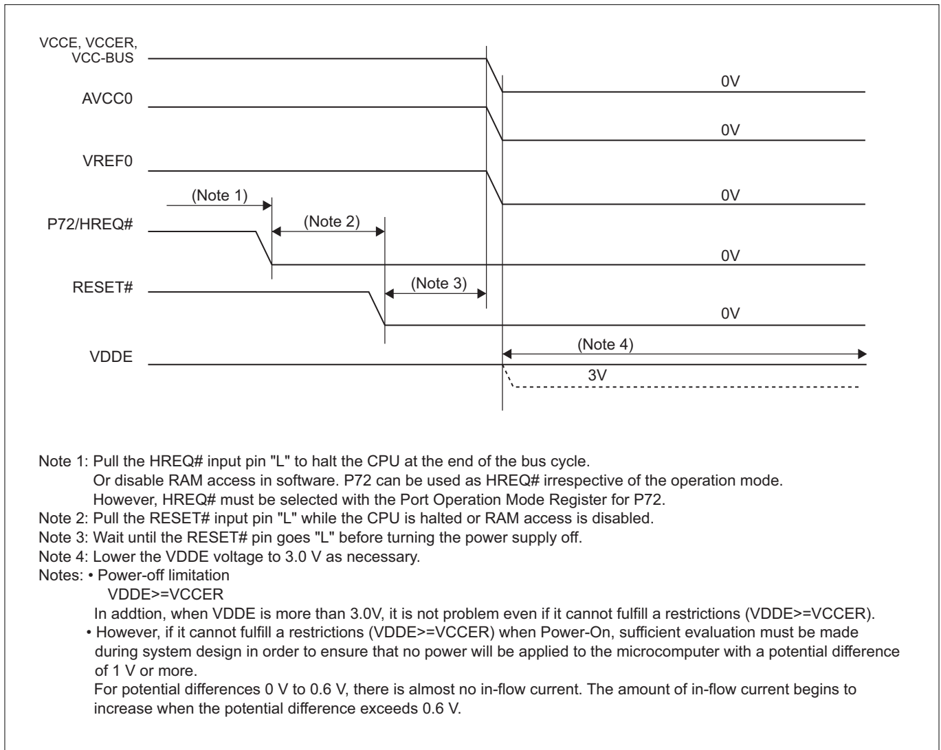
Figure 22.3.2 Power-Off Sequence when Using RAM Backup ( V_{CCE} = V_{DDE} = 5.0\text{ V} or 3.3\text{ V} )
