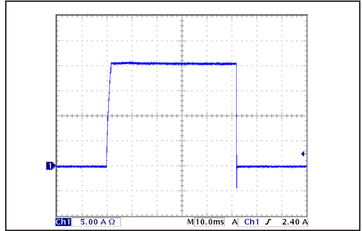
Figure 16: Load current (5A/div) as a function of time when the converter attempts to turn on into a 10 mW short circuit.
