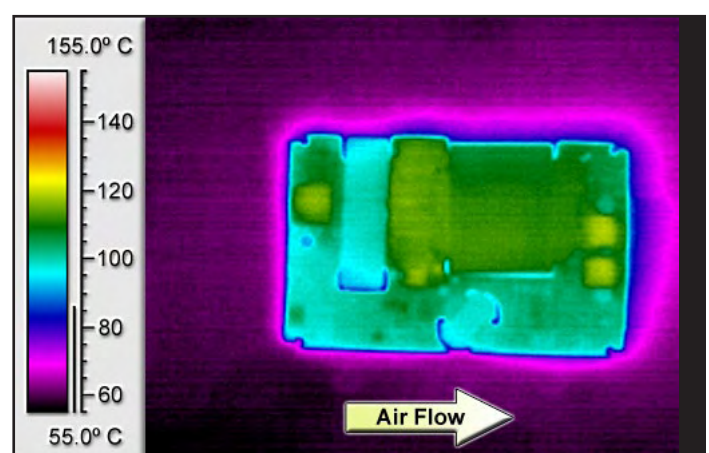
Figure 6: Thermal plot of converter at 17A load current (200 W) with 55°C air flowing at the rate of 200 LFM. Air is flowing across the converter from input to output (nominal input voltage).
