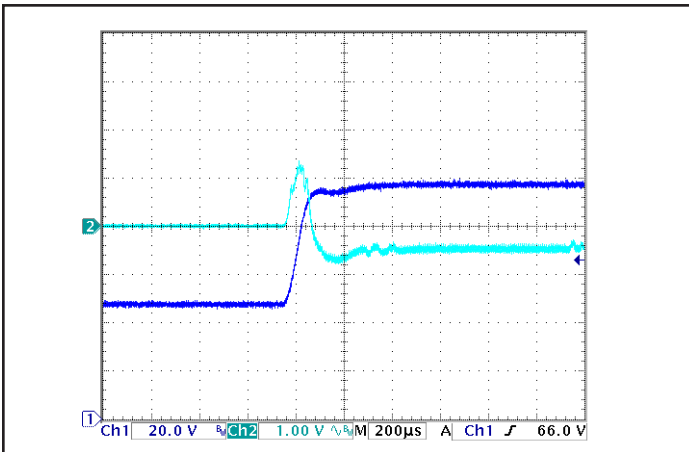
Figure 15: Output voltage response to step-change in input voltage (50V to 100V in 200μs). Load cap: 470μF, 15 mW ESR tantalum capacitor. Ch 1: Vin (20V/div), Ch 2: Vout (1V/div), at zero load current.
