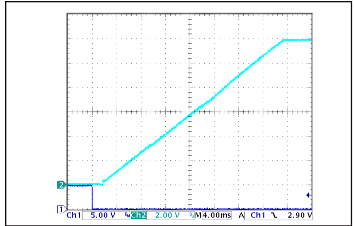
Figure 8: Turn-on transient at zero load (4ms/div). Ch 1: ON/OFF input (5V/div), Ch 2: Vout (2V/div)
