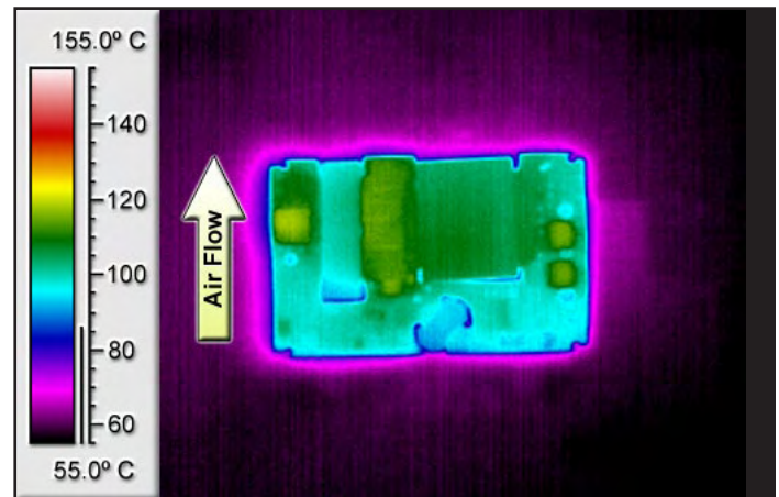
Figure 4: Thermal plot of converter at 17A load current (200W) with 55°C air flowing at the rate of 200 LFM. Air is flowing across the converter sideways from pin 1 to pin 3 (nominal input voltage).
