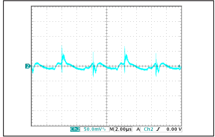
Figure 14: Output voltage ripple at nominal input voltage and rated load current (50mV/div). Load capacitance: 1μF ceramic capacitor and 10μF tantalum capacitor. Bandwidth: 500 MHz. See Figure 11.
