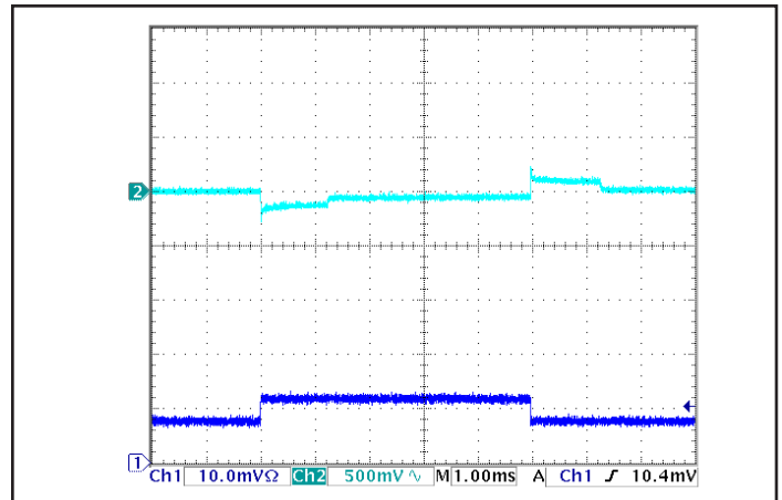
Figure 10: Output voltage response to step-change in load current (50%-75%-50% of I_{out(max)} ; dI/dt = 5A/\mu s ). Load cap: 470 \mu F , 15 mW ESR tantalum capacitor. Top trace: Vout (500mV/div), Bottom trace: Iout (10A/div).
