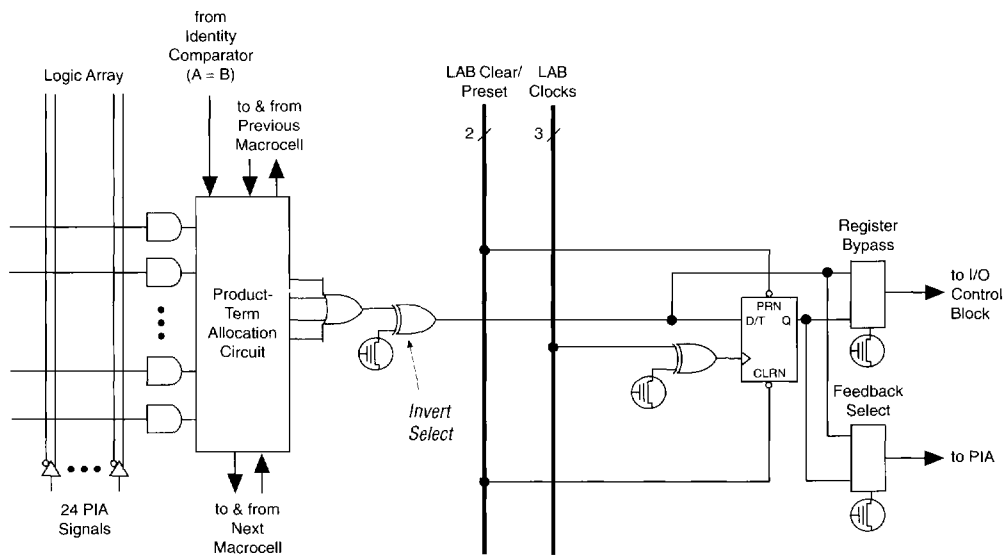
Figure 3. FLASHlogic Macrocell
