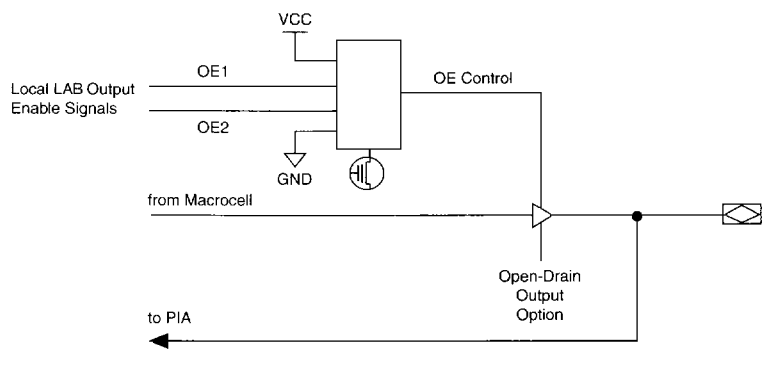
Figure 7. I/O Control Block for FLASHlogic Devices
