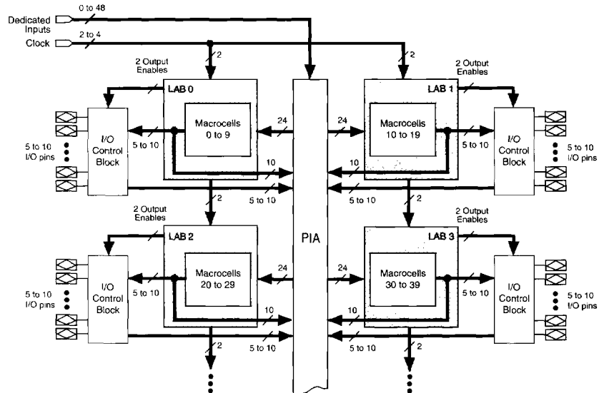
Figure 1. FLASHlogic Architecture
