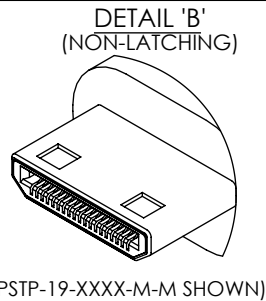
(HPSTP-19-XXXX-M-M SHOWN)
