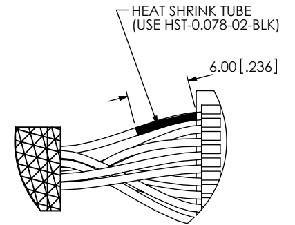
HEAT SHRINK DETAIL DETAIL 'D' SCALE 2:1
