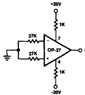
Burn-In Circuit
