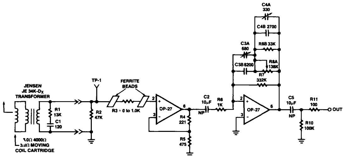
Figure 1. RIAA Phono Preamplifier
