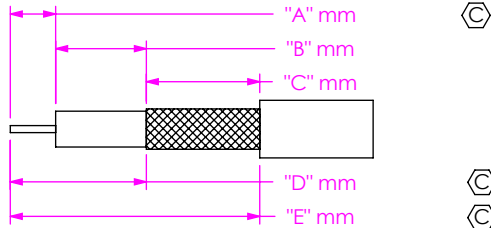
FIG. 2 CABLE STRIPPING DIMENSIONS PER CONFIGURATIONS (SEE TABLE 1) (SEE NOTES 12,13,14,15)
