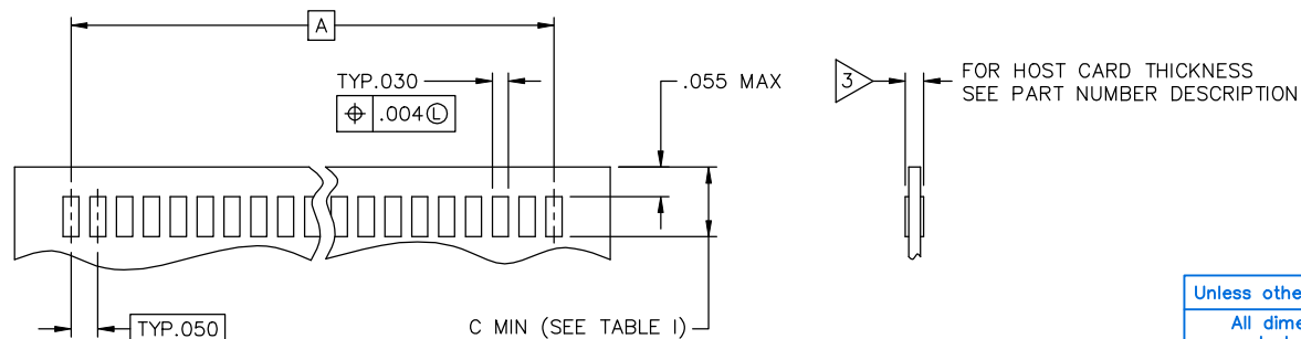
RECOMMENDED HOST CARD LAYOUT
