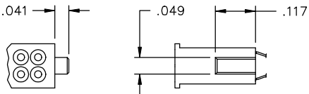
TSB-____ [2] _ 4 D-00 _ (NARROW EAR)
