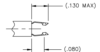
TSB-____ [3] 4 D-00 9 (MINIMIZED CENTRAL STRADDLE - .062 PC CARD ONLY)
