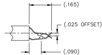
TSB-____ [2] 4 D-00 _ (OFFSET STRADDLE)
