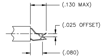
TSB-____ [4] 4 D-00 _ (MINIMIZED OFFSET STRADDLE)
