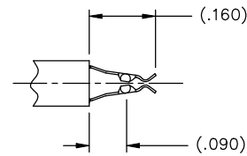
TSB-____ [1] 4 D-00 _ (CENTRAL STRADDLE)
