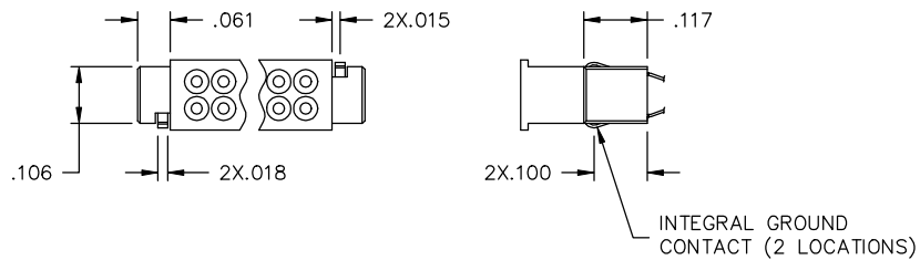
TSB-____ [3] _ 4 D-00 _ (FULL EARS W/ INTEGRAL GROUND CONTACTS)
