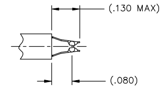
TSB-____ [3] 4 D-00 _ (MINIMIZED CENTRAL STRADDLE)
