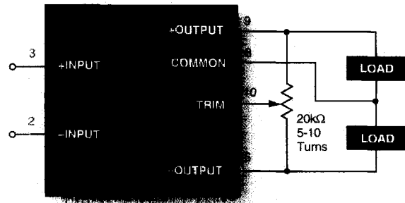
Figure 8. Trim Connections Using a Trimpot
