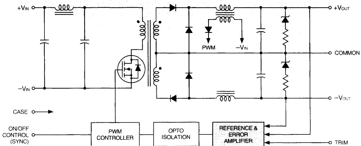
Figure 1. Simplified Schematic
