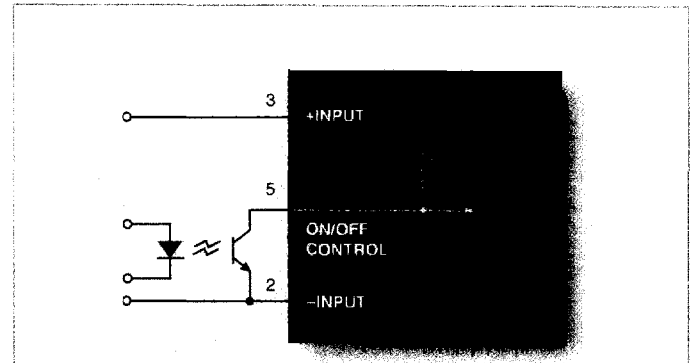
Figure 6. Driving the On/Off Control Pin
