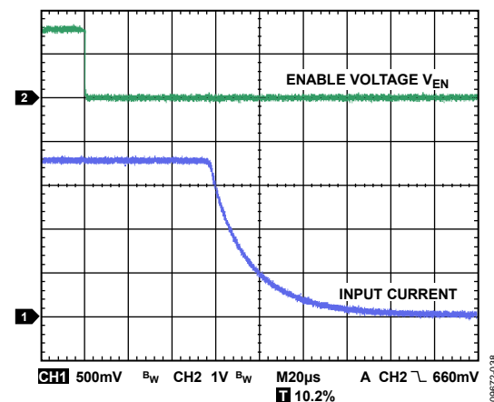
Figure 38. Typical Turn-Off Time
