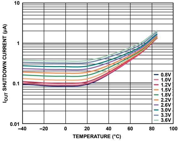
Figure 16. Output Shutdown Current vs. Temperature, V_{OUT} = 0V , Different Input Voltage ( V_{IN} )
