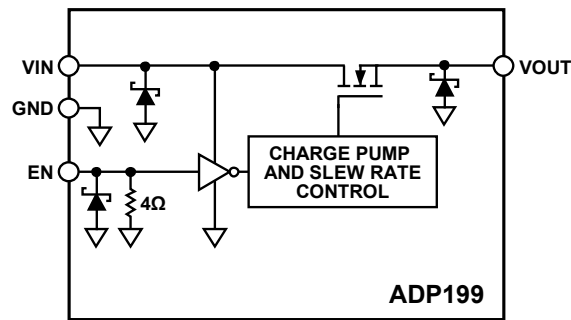
Figure 29. Functional Block Diagram
